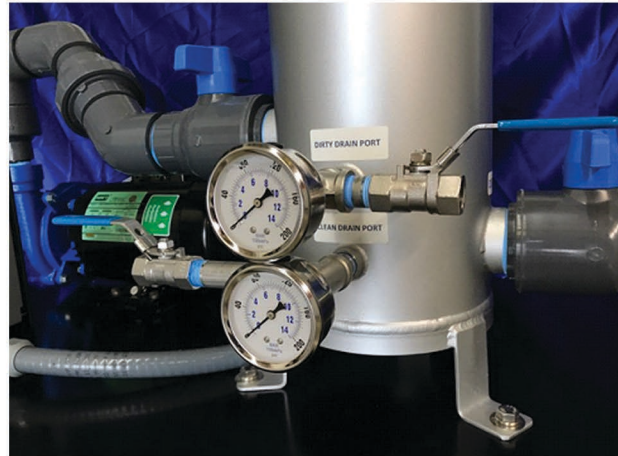
Pressure Gauges and Drain Valves
